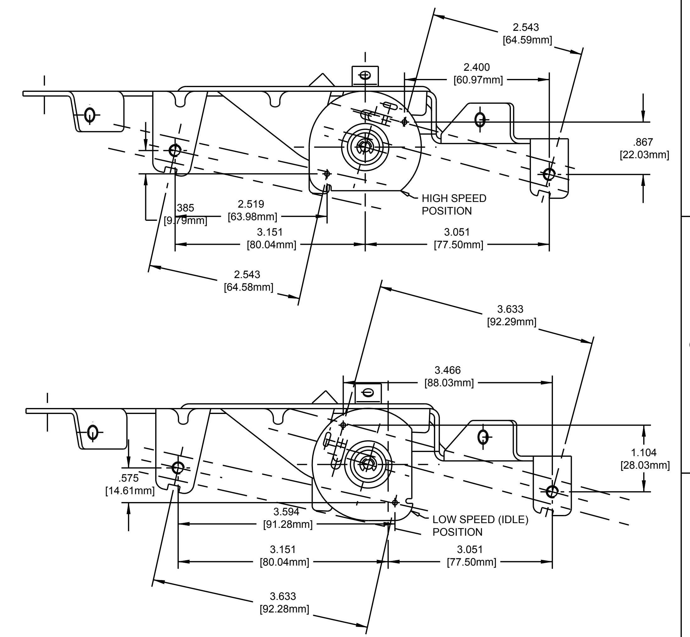
THROTTLE CONTROL BRACKET REFERENCE INFORMATION. SEE SHEET 10 FOR CUSTOMER THROTTLE CABLE ATTACHMENT LOCATIONS FOR ENGINES WITH FUEL TANK
