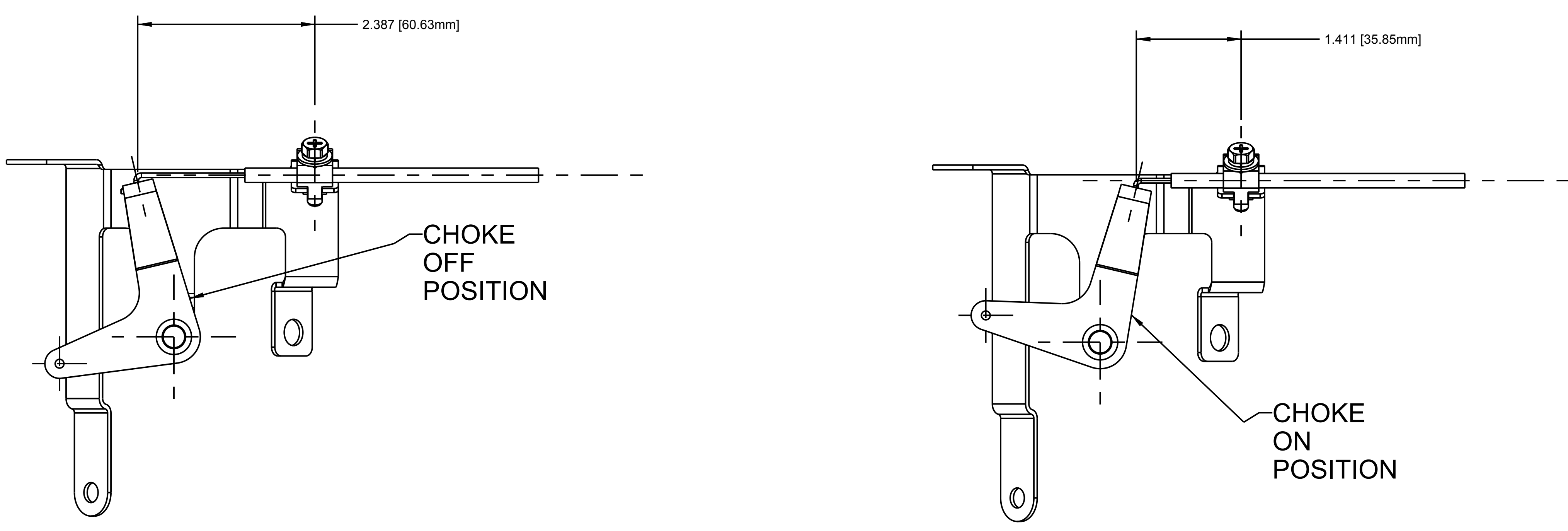
REMOTE CHOKE CONTROL BRACKET
